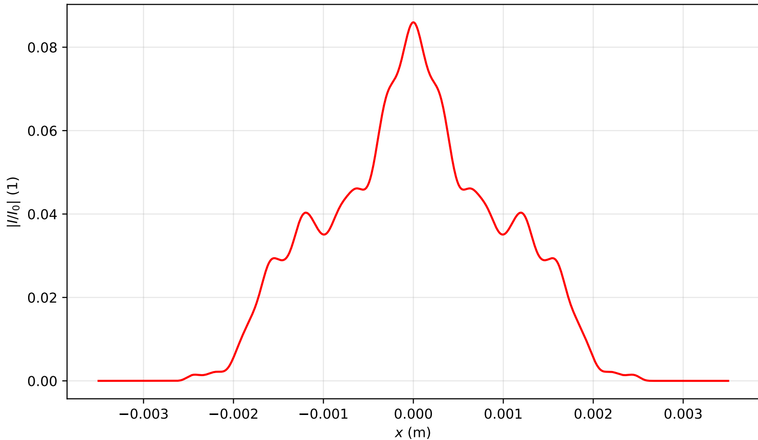
Intensity profile I(x, y = 0, z = 3.582)/I_0 , P_{in}=5.5P_{cr} , artificial time
